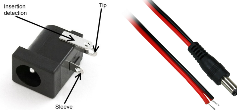
Figure 21 - DC power jack female (left) and male (right) connectors [29, 30]
