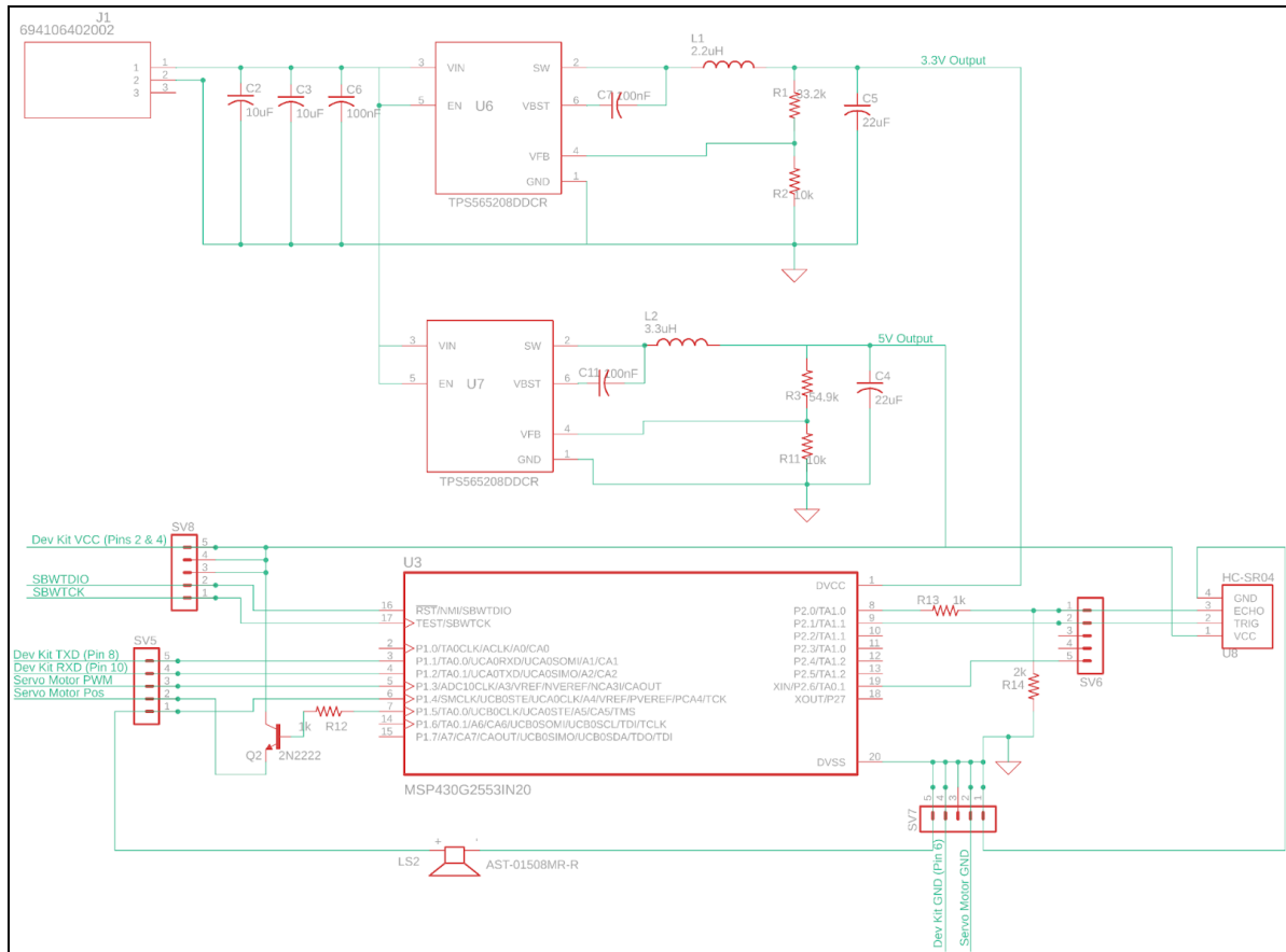
Figure 20 - Overall schematic
