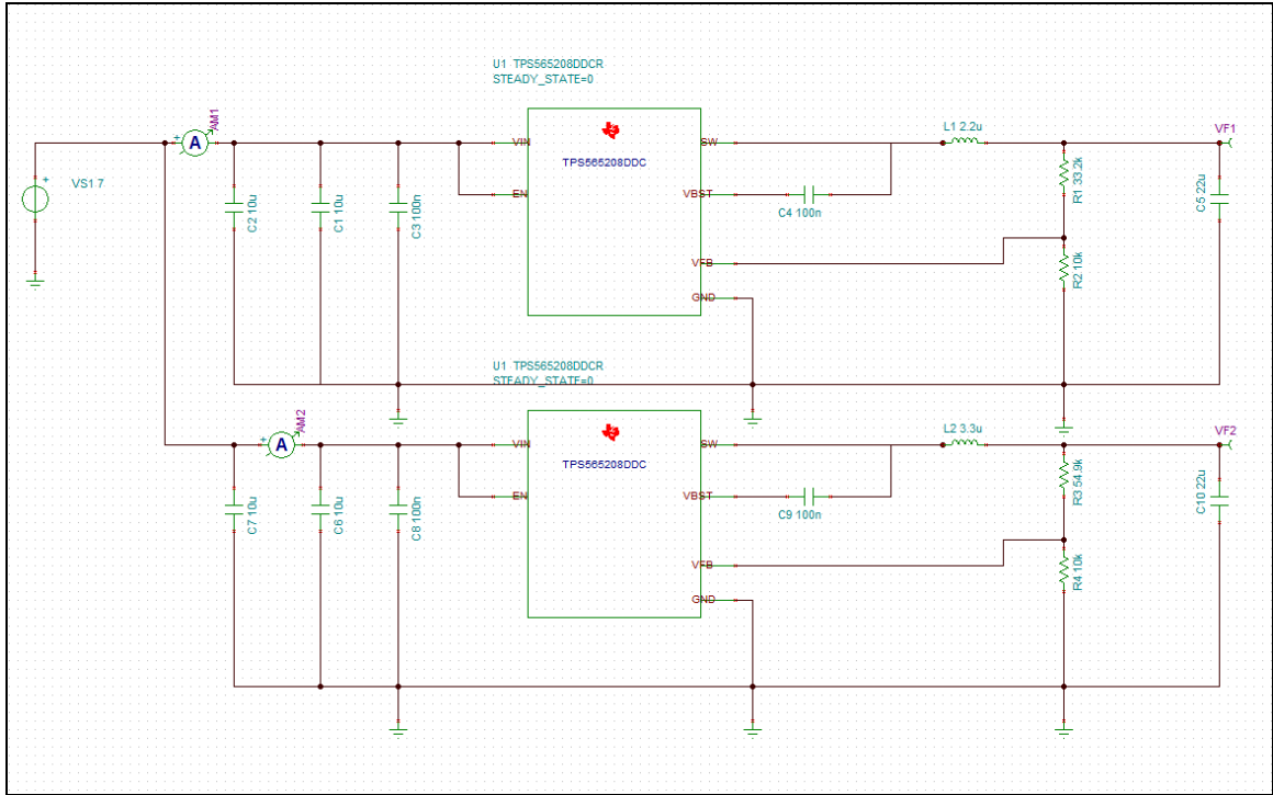
Figure 12 - 3.3V and 5V voltage regulator designs
