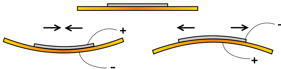
Figure 7 - Piezoelectric Effect [27]
