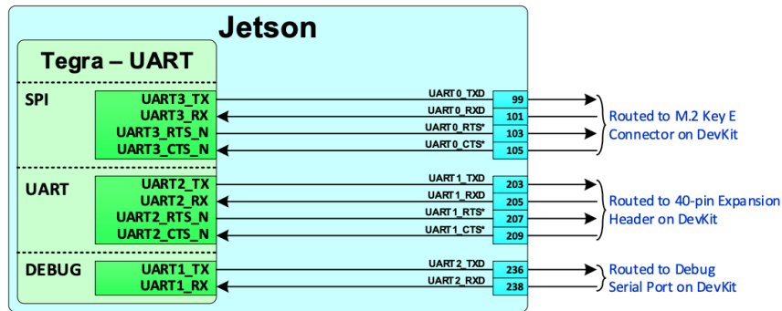
Figure 13 - Jetson Nano UART connections
