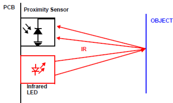
Figure 6 - Infrared LED to proximity sensor behavior diagram [25]
