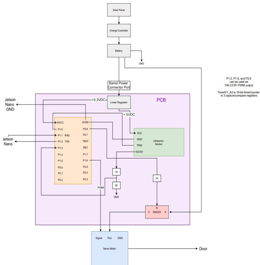
Figure 8 - PCB to servo motor block diagram
